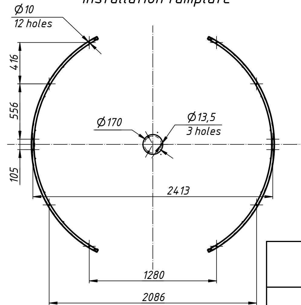
Installation tamplate
