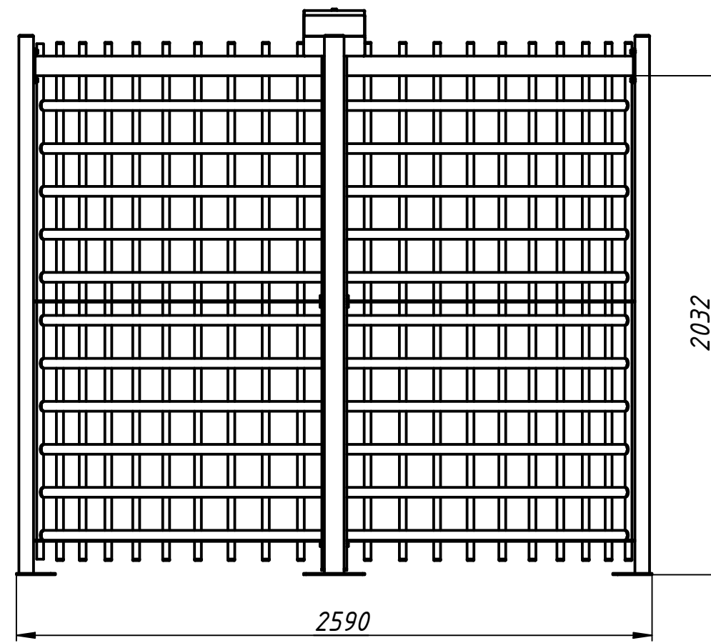
Installation tamplate
