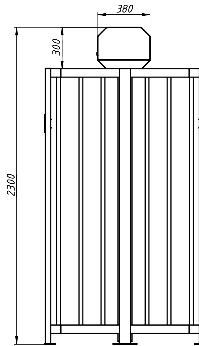
Instalation tamplate
