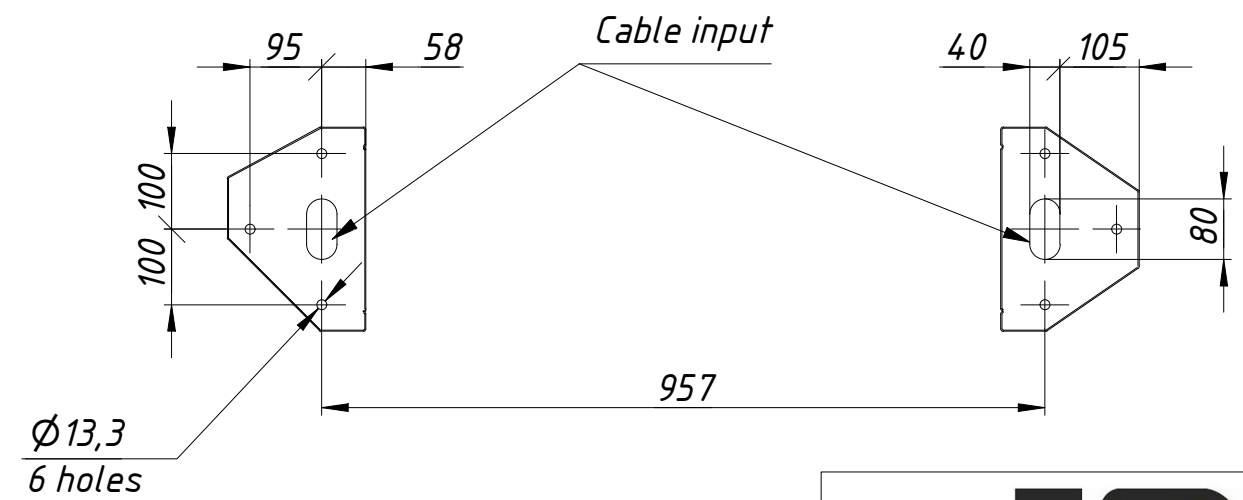
Installation tamplate
